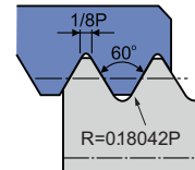
ISO 5855-1999 Tolerance: 4
