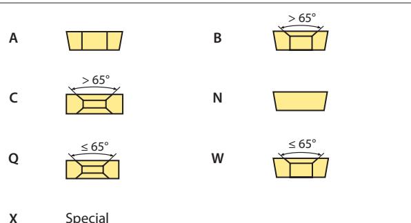
Insert shape
