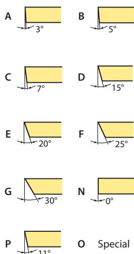
Clearance angle
