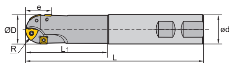
Weldon shank
